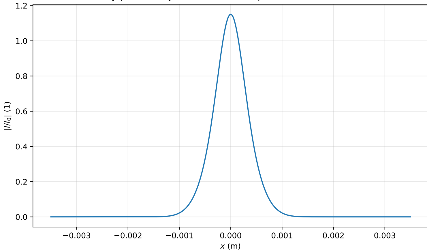
Intensity profile I(x, y = 0, z = 0.716m)/I_0 , P_{in}=0.7P_{cr} , artificial time
